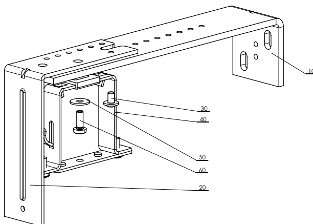
Adjustable bracket – fixed 256 – 318 mm P 010/43 (2-01801-0000)
