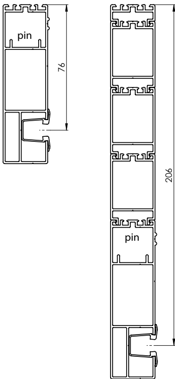
Basic profile P 020 Maximum possible expansion of the basic profile P 020 Basic profile P 080 Maximum possible expansion of the basic profile P 080 Basic profile P 081 Maximum possible expansion of the basic profile P 081
