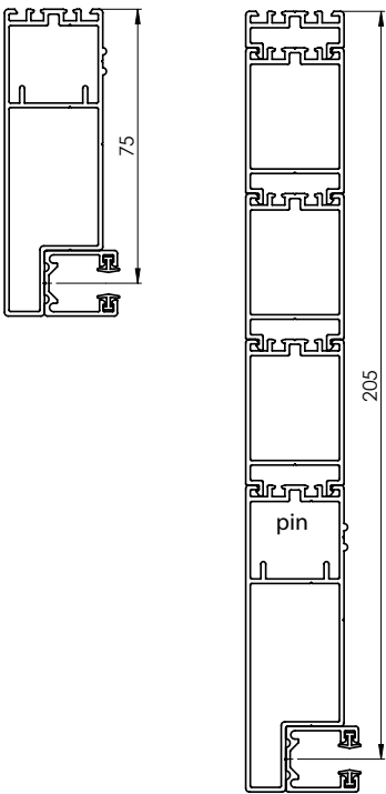
Basic profile P 020 Maximum possible expansion of the basic profile P 020 Basic profile P 080 Maximum possible expansion of the basic profile P 080 Basic profile P 081 Maximum possible expansion of the basic profile P 081
