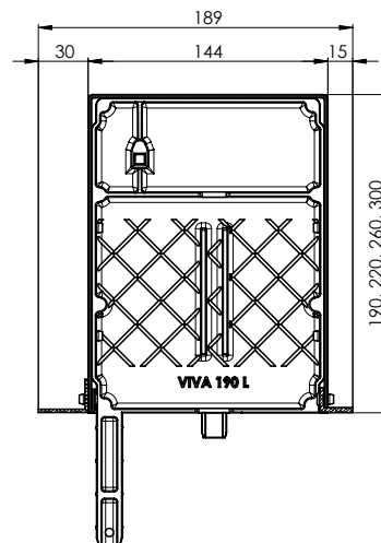
Cross-section of under-plaster VIVA box + P 020/03, P 080/03, P 081/03
