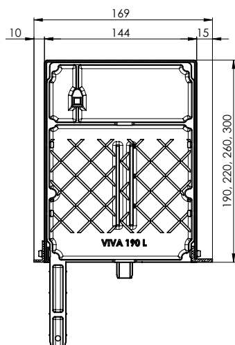
Cross-section of under-plaster VIVA box + P 020/01, P 080/01, P 081/01
