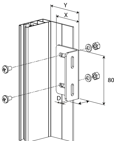
Distance support for guide rail 828 and 828 and 838:
