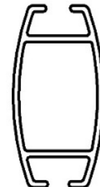
Bottom rail AL - fabric cover RBR/1 (7-302578)
