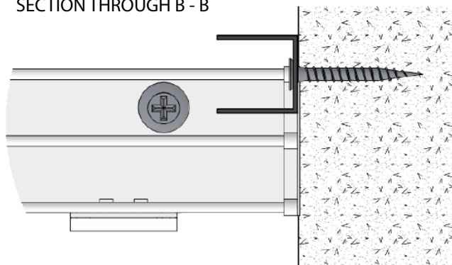
SECTION THROUGH B - B
