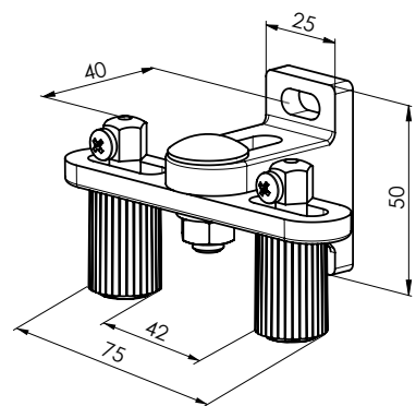
Double cable guide, 70 - 130 mm P032/8 (2-01652)
