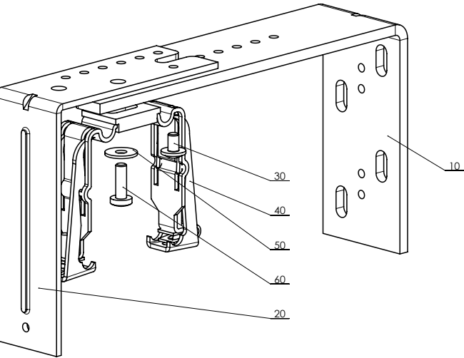
Adjustable double bracket - mechanical 306 – 368 mm P 010/41 (2-01799-0000)
