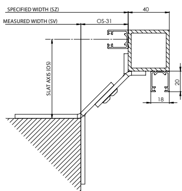
Measurement - channel
