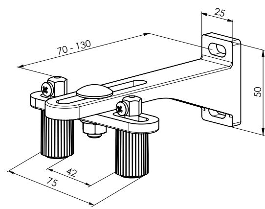
Double cable guide, 70 - 130 mm P032/8 (2-01652)
