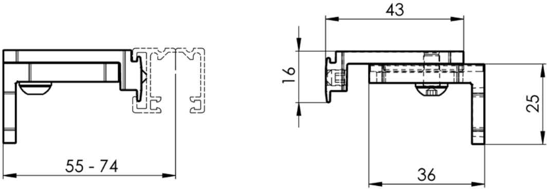
Guiding channel holder 055 - 74 mm Zn P021/50 (2-01818-PU11)
