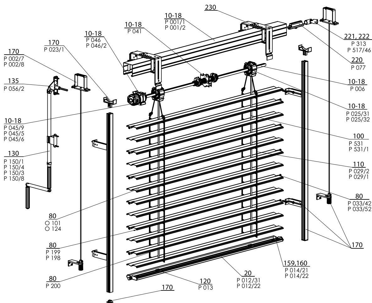
ZETTA 70/90 - HANDLE 2-00157-XXXX-G
