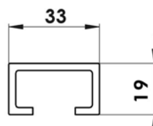
Guide rail (6-008727)
