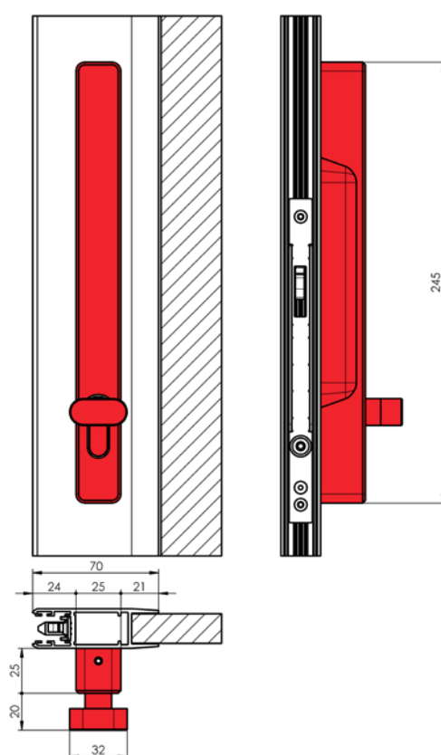
Handle with lock, knob control
